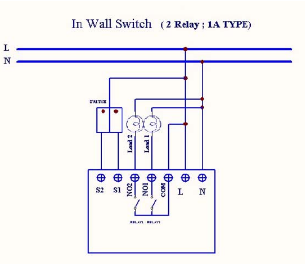
Fig 1. Assembling
